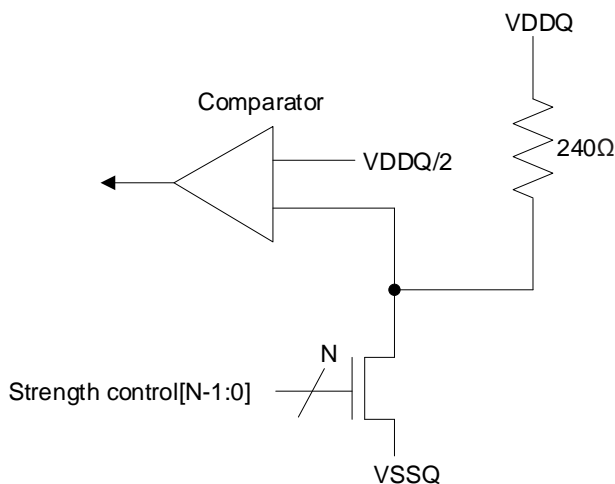
Figure 5-19 Pull-down Calibration
