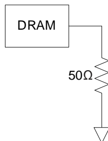
Figure 5-17 Driver Output Reference Load for Timing and Slew Rate
